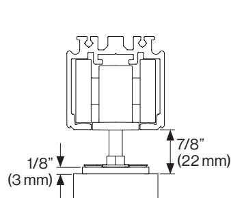
Maximum Clearance
