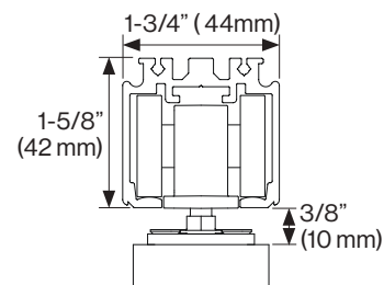
Minimum Clearance
