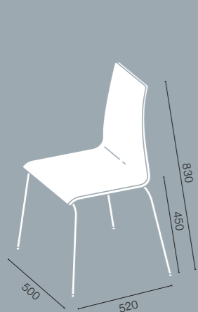
565GK-10 Comfort plastic seat shell
