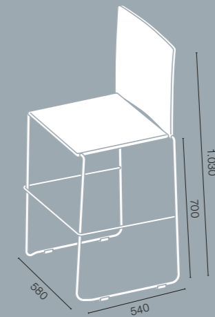
546BU-10 Comfort plastic seat shell
