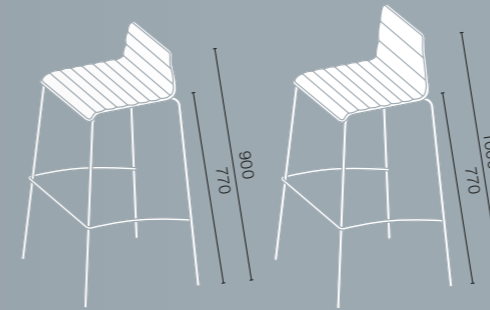
4-leg barstool, metal | 4-leg barstool, metal
