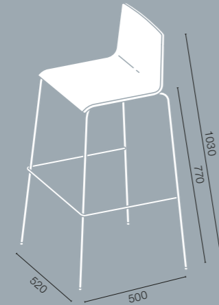
8519-10 Comfort wooden seat shell, barstool
