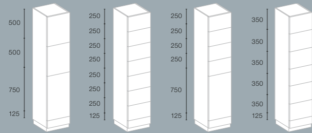
Locker cabinets FD | FDS Available in 4OH and 5OH heights
