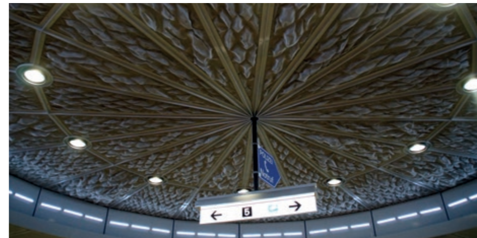
Three-dimensional stainless-steel mesh for improving the space's acoustics. Cologne light railway, Germany, MONTANA.
