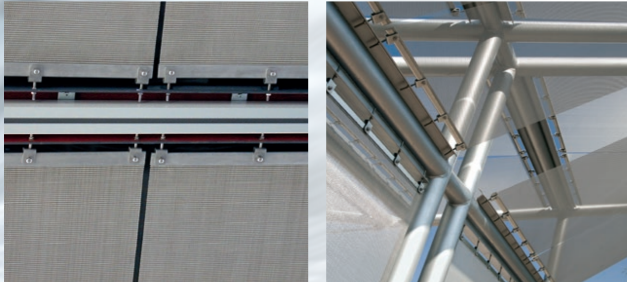
Fixed mounting system for ceiling with flat tension profiles and clevis screws.
