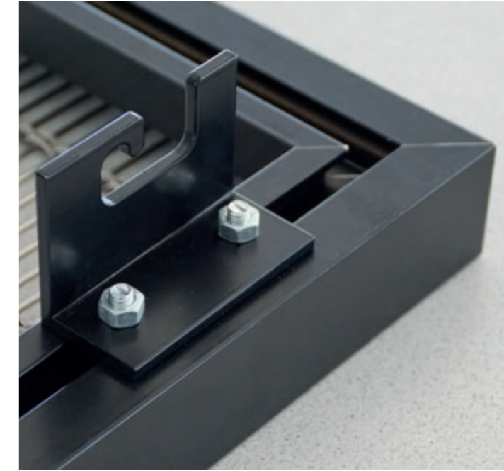
Special version: Hanging options for framed elements.
