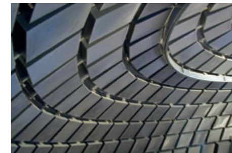
Cassette elements with acoustic fleece. Print Media Academy, Heidelberg, Germany, DETENTION.
