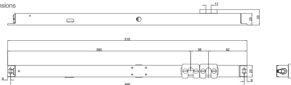
Emergency unlocking tool part. No. 41596Q
