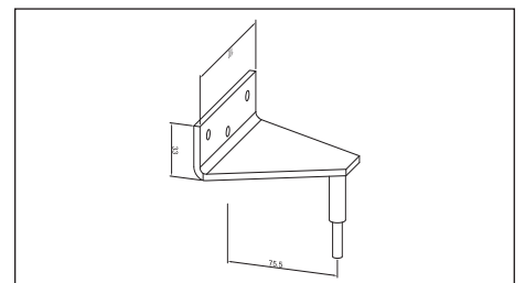
Short triangular bracket (75,5 mm) part No. 41924F Long triangular bracket (150 mm) part No. 41923E
