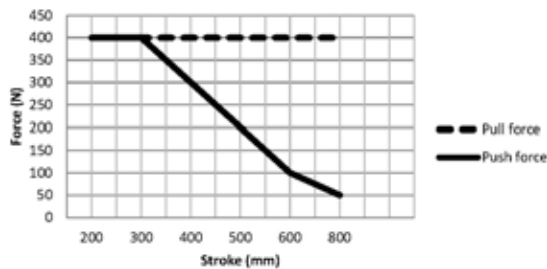
Stroke/force diagram
