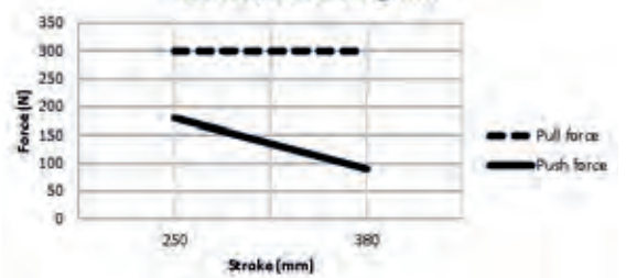
Stroke/force diagram
