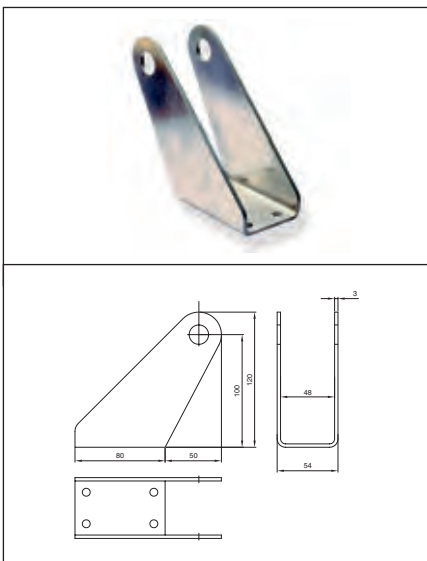
Aluminium front bracket part No. 356960 It allows the fixing of the cylinder to the frame and the cylinder rotation during the opening phase. The bracket is connected to the cylinder by pivot or nipples.
