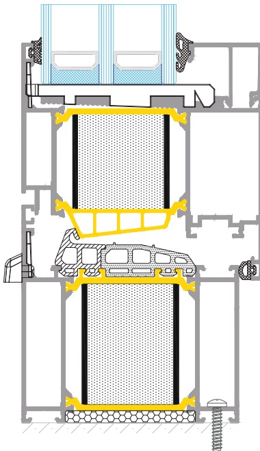
A KESİTİ SECTION A
