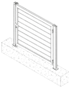
tek kanat kapı single sash door
