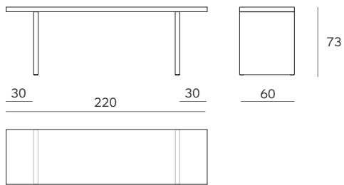
Mod. 0662-01
