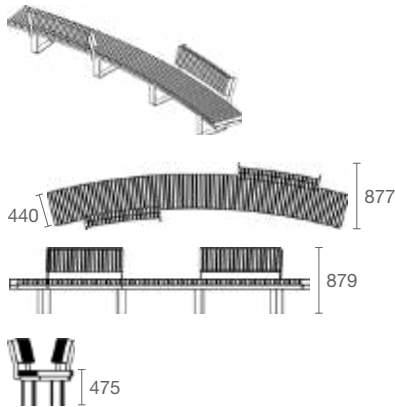
3 Curved module
