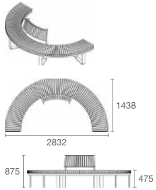
5 Half-circle module
