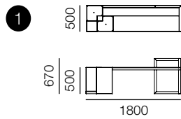
BANQUETTE BACKLESS BENCH
