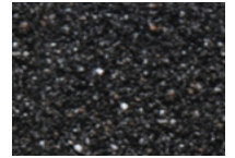
GRAPHITE NEBULA
