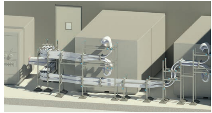
nVent CADDY Pyramid H-Frame and nVent ERIFLEX Flexbus Installation
