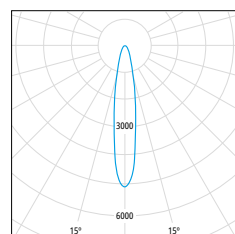
SPOT 18°
