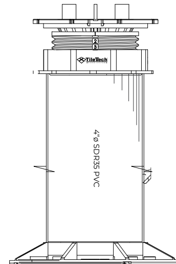
Uni-Just™ w/ PVC Pipe Height: "Variable" Max 54" (with Lateral Bracing and Tray System). Slope: 0% TO 4%
