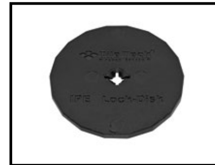
IPÊ Lock Disk: Used to secure wood tiles by inserting disk into kerf-cut between the upper slat and bottom rail, adding the 4th tile and securing with 1-1/4" deck screw.
