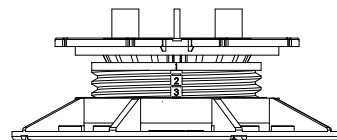
Uni-Just™ w/o PVC Pipe Height: 2-1/4" To 3" Slope: 0% To 4%
