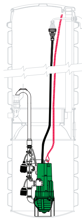
MODEL 6923 - FREE STANDING
