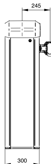
Front view
