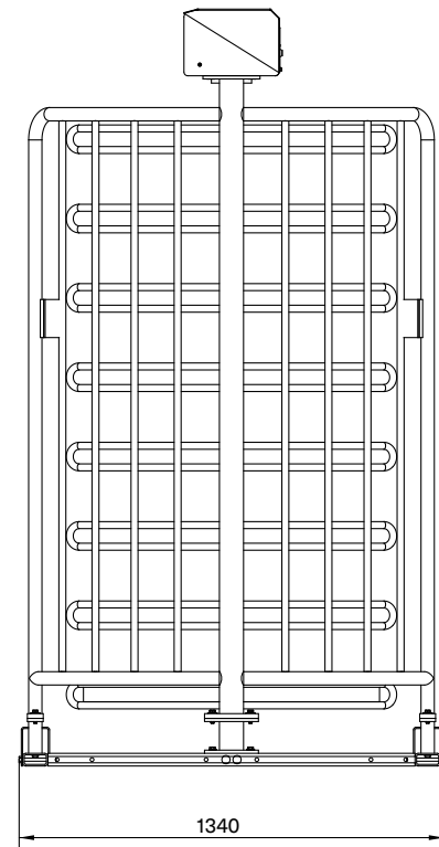
MPT *3* pre-assembled – view from the side
