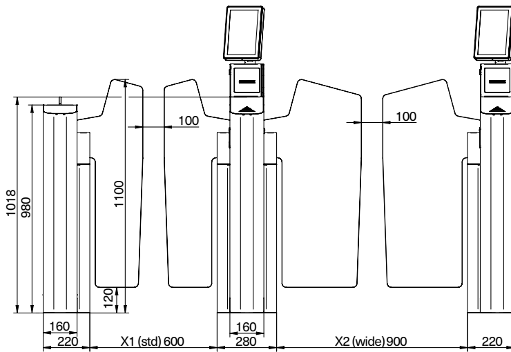
mGo (2-line configuration) – front view
