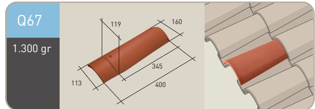
Remate lateral curvo derecho
