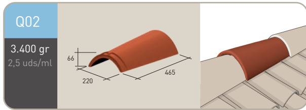
Remate curva 50
