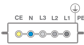
3L+N+CE+PE(Housing) 3 Phase / Clean Earth
