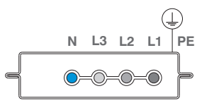
3L+N+PE(Housing) 3 Phase System
