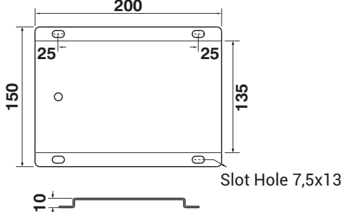
Floor "U" Support Details
