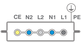
2L+2N+CE+PE(Housing) Dual Circuit Busbar
