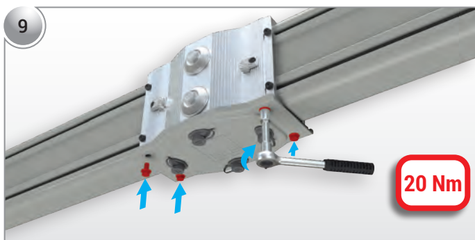
Torque the bolts of the lower block joint cover to 20 Nm.
