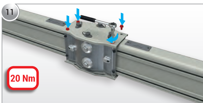
Install the top block joint cover and torque its bolts to 20 Nm.
