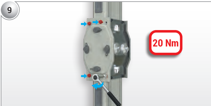
Install the other block joint cover and torque its bolts to 20 Nm.
