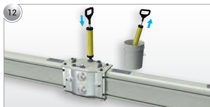
Ensure the injection piston is fitted to prevent leakage at the casting opening and inject Flex-Comp material into the block joint cavity using a lever. Continue injection until Flex-Comp is visible from the other end. Close the plastic cover and finalize the installation.
