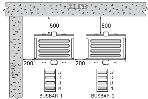
Figure 3 - Flatwise Application
