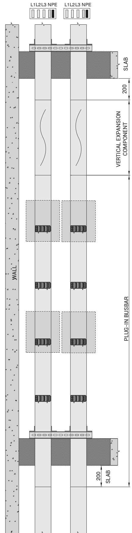
FIGURE-9 MINIMUM DIMENSIONS ON SHAFT APPLICATIONS
