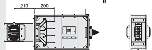
Feeder Box sample equipped with MCCB
