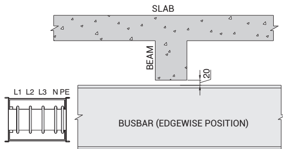
FIGURE-7 CROSSING UNDER A BEAM EDGEWISE POSITION
