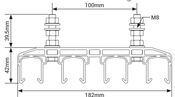
Plastic Sliding Hanger (Quad)
