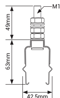
Steel Sliding Hanger
