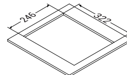
NDK-CX 2 (24 Module) Floor Cut Size
