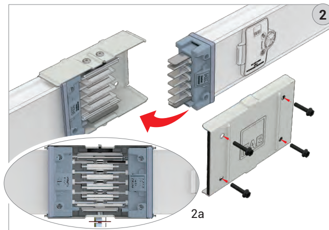
Align two busbars like the picture-2a and insert the busbar conductors into the block joint.
