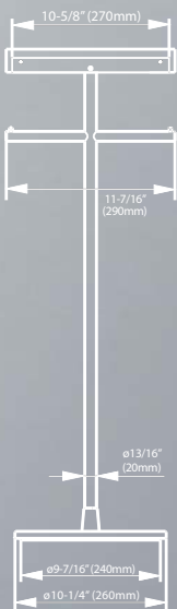
NEOREST REMOTE CONTROL STAND; YS990
