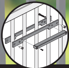
Mounting Plate for Guide Rail DCAC632-9004
