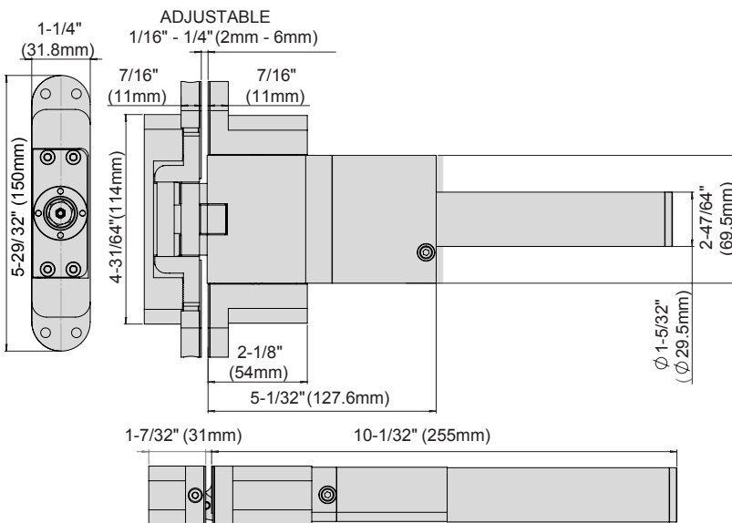
77108523 CLOSER + HINGE
