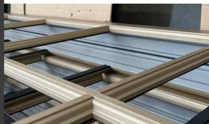
Reparto estrusione profili in alluminio | Aluminium profiles extrusion department
