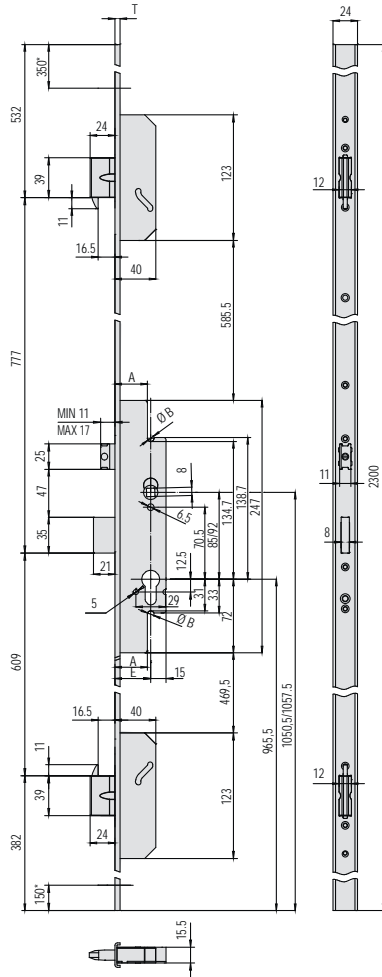
49526, 49726, 49728 49436, 49636, 49638 49426, 49626
