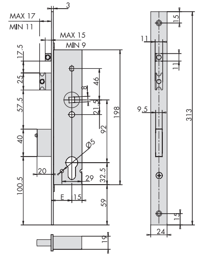
43225, 43235, 43236 E = 30-35-40-45
