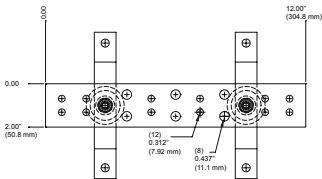
13622-012: (16) Lugs, 5/8" (15.88 mm) hole centers (3) Lugs, 1" (25.4 mm) hole centers
