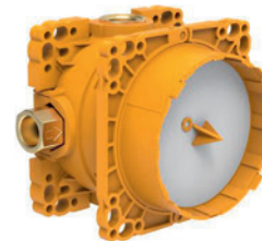
HF574037000000 Concealed box, for bath and shower mixers, fittings 1/2", with stopvalves
