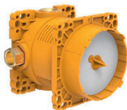
HF574007000000 Concealed box, for bath and shower mixers, fittings 1/2", with stopvalves, inversion for in-/outlets possible
