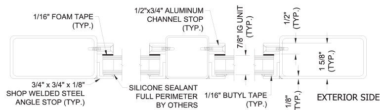
INSIDE SASH RETAINER ASSEMBLY - UP TO 15/16" INSERTS NO SCALE
