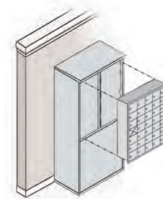
ENCLOSURE DISPLAYED WITH 7 DOOR HIGH RECESSED MOUNTED CELL PHONE LOCKER
