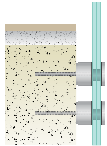
1 WITHOUT OVERHANG/ SANS REBORD External fixing/ Fixation extérieure
