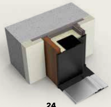
24 Controtelaio e telaio per porta blindata a bilico Di.Big per posa in tunnel. Subframe and frame for Di.Big pivot security door for installation on straight walls.
