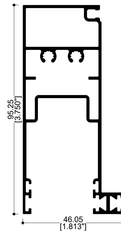
70949 Zoclo mosquitero
