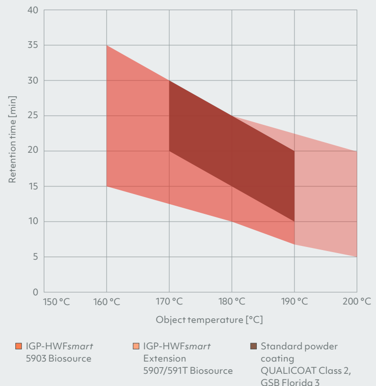
Extended curing window of IGP-HWFsmart 59 Biosource compared to conventional super durable façade powder coatings (QUALICOAT Class 2, GSB Florida 3)
