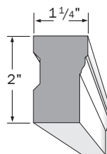
Brick Mould PCBBRICKMOULD - 18'
