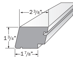
Heavy Sill Nose PCBHEAVYSILLNOSE
