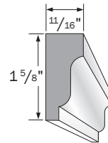
Shingle Mould PCBSHINGLEBAND
