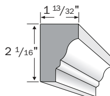
Rams Crown PCBRAMSCROWN
