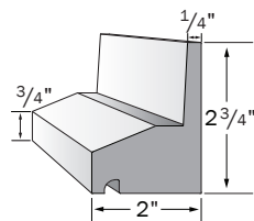
Water Table PCBWATERTABLE - 18'
