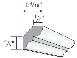
Bed Mould PCBBEDMOULD
