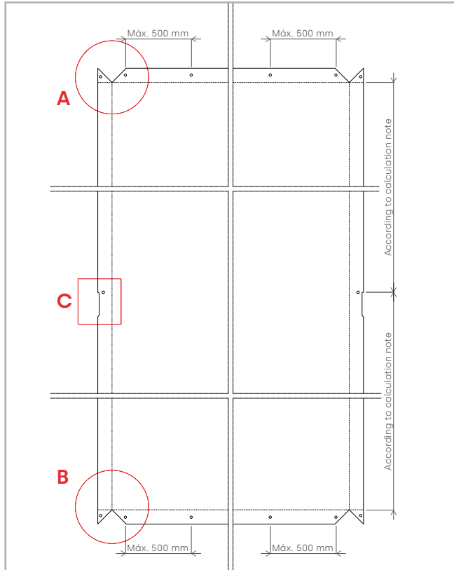
UNFOLDED CASSETTE
