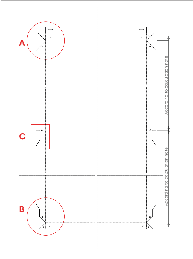
UNFOLDED CASSETTE
