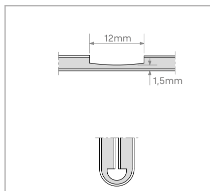
*Arc milling groove for complete 180° folds.
