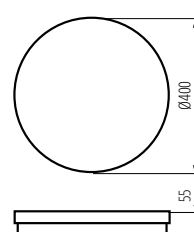
BENO ECO 40W CCT O
