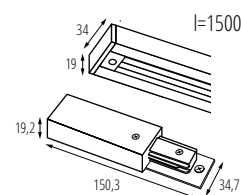
TEAR 1F SET 1,5M-B
