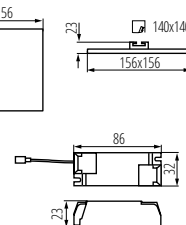
AREL LED DL 14W
