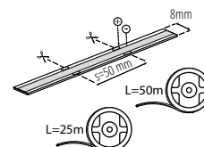
LCOB 3W/M 24 IP00
