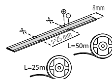
LCOBB 3W/M 12 IP00
