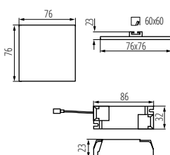
AREL LED DL 6W
