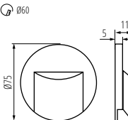
ERINUS LED O
