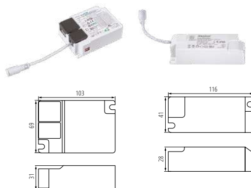
BLINGO DRVM24W ON-OFF 37262 BLINGO DRVM34W ON-OFF 37263 BLINGO DRVM42W ON-OFF 37264
