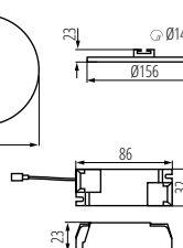
AREL LED DO 14W
