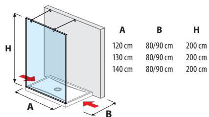
glass wall fixed 120, 130, 140 cm
