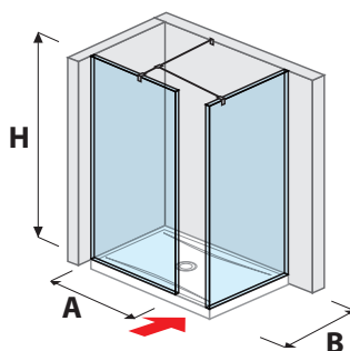
glass wall/walk in PURE corner version for shower trays 70, 80 x 80 cm | 70, 80 x 90 cm
