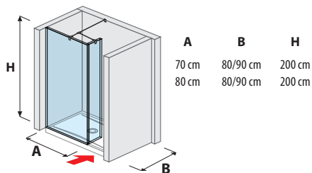
glass wall incl. short glass 70, 80 cm
