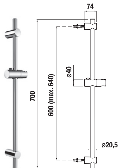
Variable slide bar mounting system
