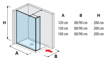
glass wall incl. short glass 120, 130, 140 cm
