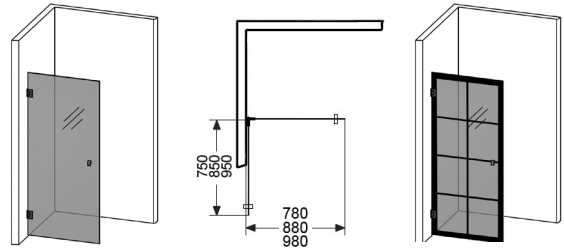
180° Rista with industrial decor.
