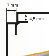
Internal corner
