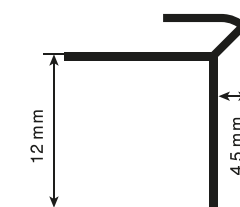
External corner
