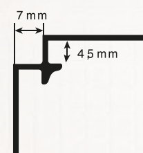
Internal corner
