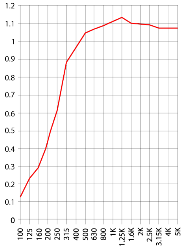
SOUND ABSORPTION REPORT RAL-A17-297
