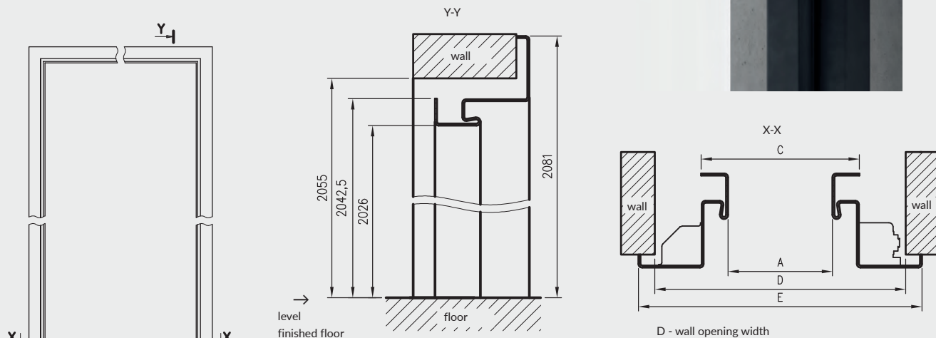
Dimensions for single leaf doors
