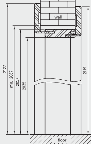
vertical cross-section of adjustable tunnel with T80 architrave
