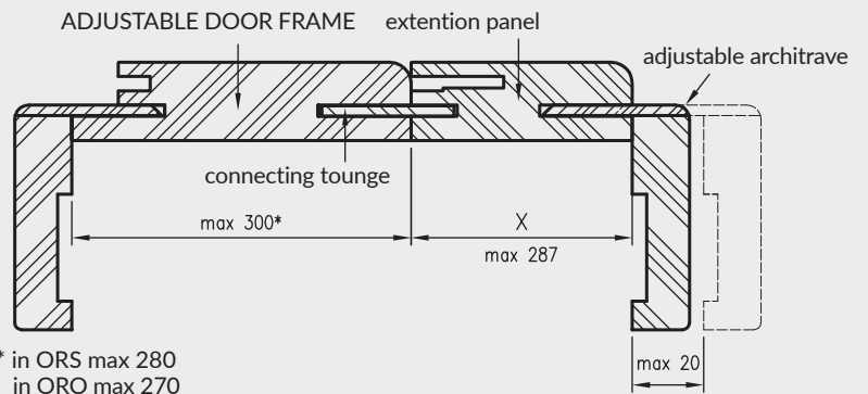
options of the width of panels cross-section
