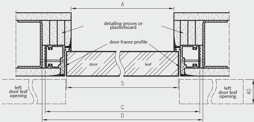
Horizontal cross-section of the Sara Eco 2 non-rebated door - opening outwards
