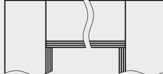
Adjustable door frame connection at an angle of 90° T80 architrave
