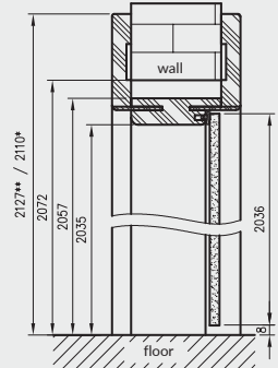
vertical cross-section of glass doors with ORC
