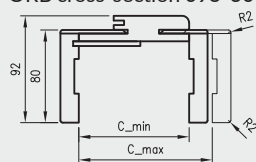
ORB cross-section 075
