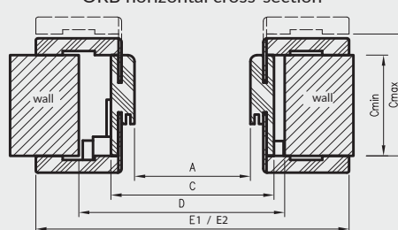
ORB horizontal cross-section
