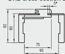
ORB cross-section 075
