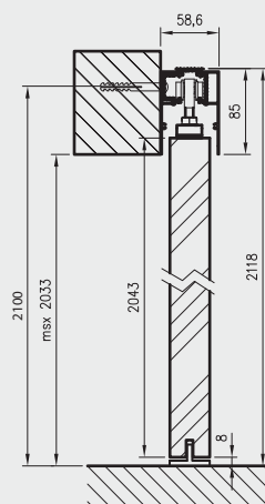
vertical cross-section
