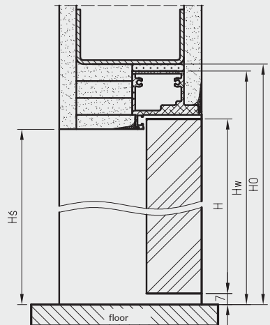
DRE profile for non-rebated outward opening doors
