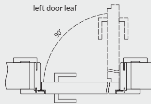
horizontal cross-section of ORO
