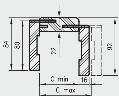
tunnel cross-section with T63 architrave
