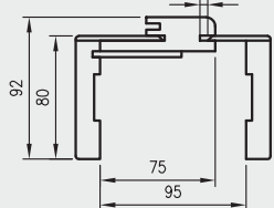
ORB cross-section 075
