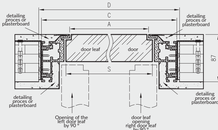
Cross-section of 50mm inverted rebate door - opened inwards
