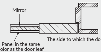
Estra 10 door in the "reverse" variant
