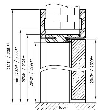
vertical cross-section
