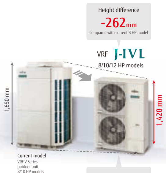
Image: 8/10/12 HP models
