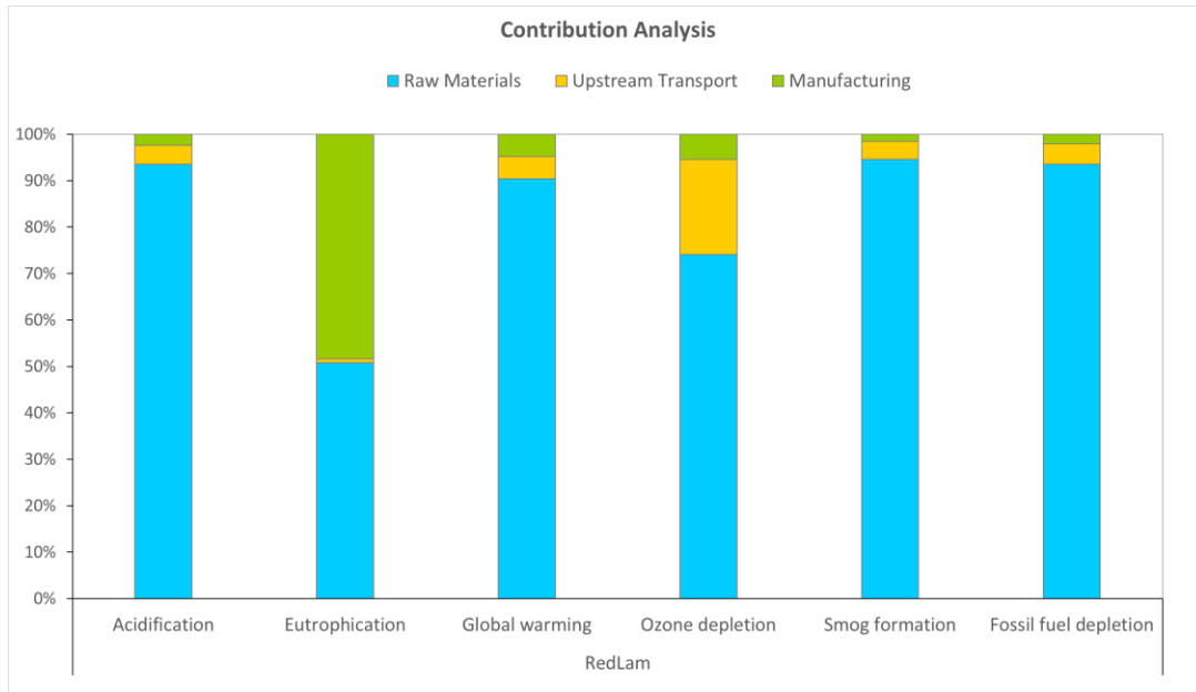
Figure 4. Contribution analysis for the Redbuilt™ RedLam™ LVL products.
