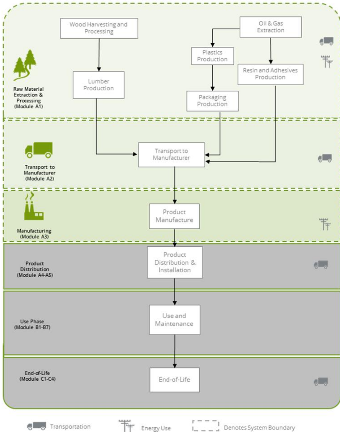
Figure 1. Flow Diagram for the life cycle of the RedBuilt™ product system.
