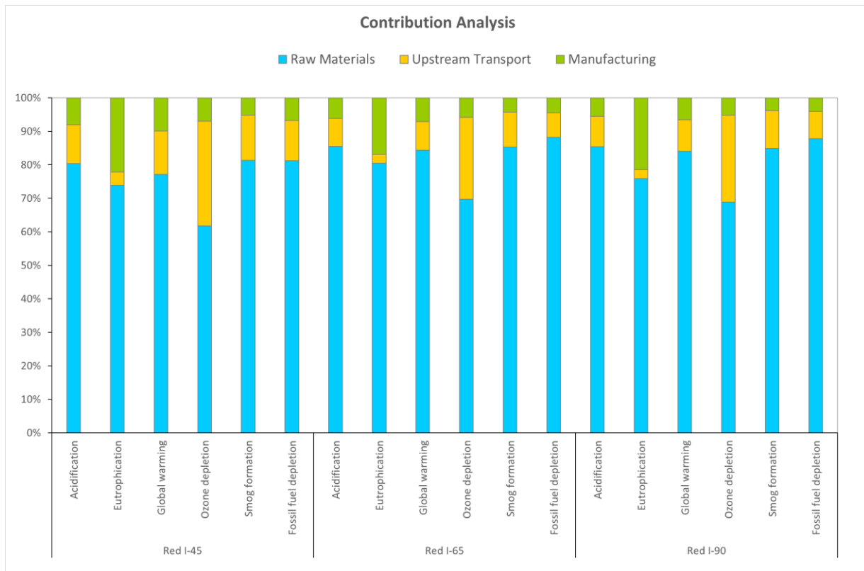
Figure 5. Contribution analysis for the Redbuilt Red-I™ Joist products.
